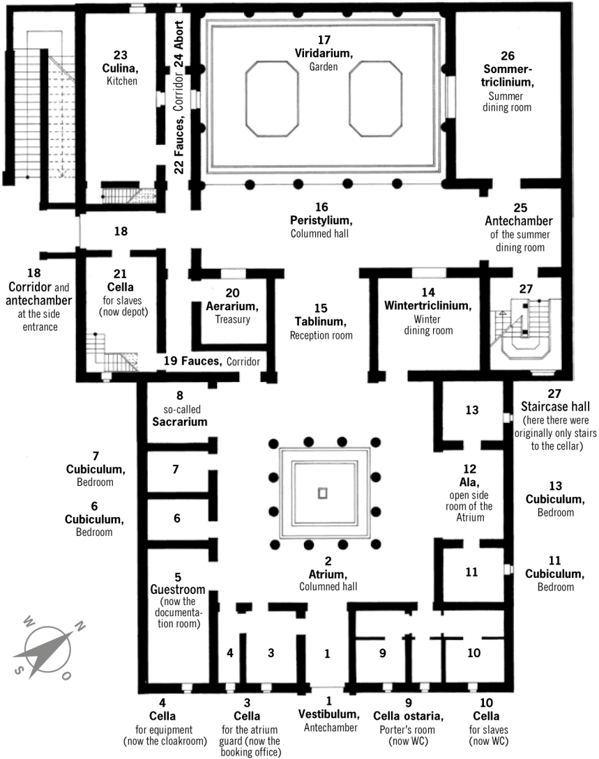
Ground plan of the ground floor
