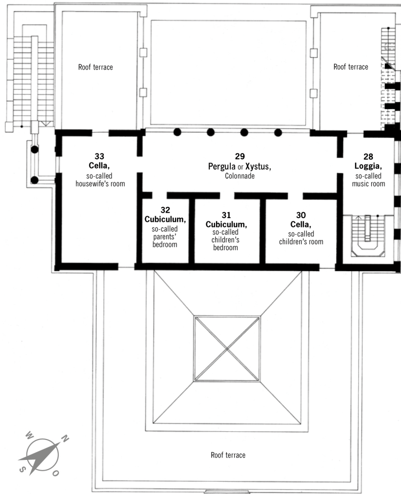
Ground plan of the first upper floor
